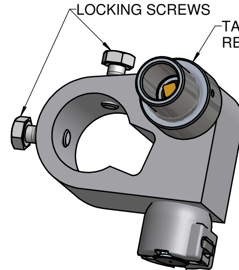
S51234 RESTRICTOR BLOCK ASSEMBLY
